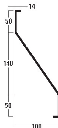
B300-BP (Louver 300)
