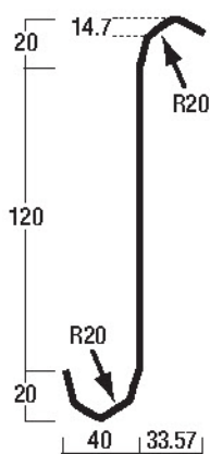
B160-PL (Louver S PLUS)
